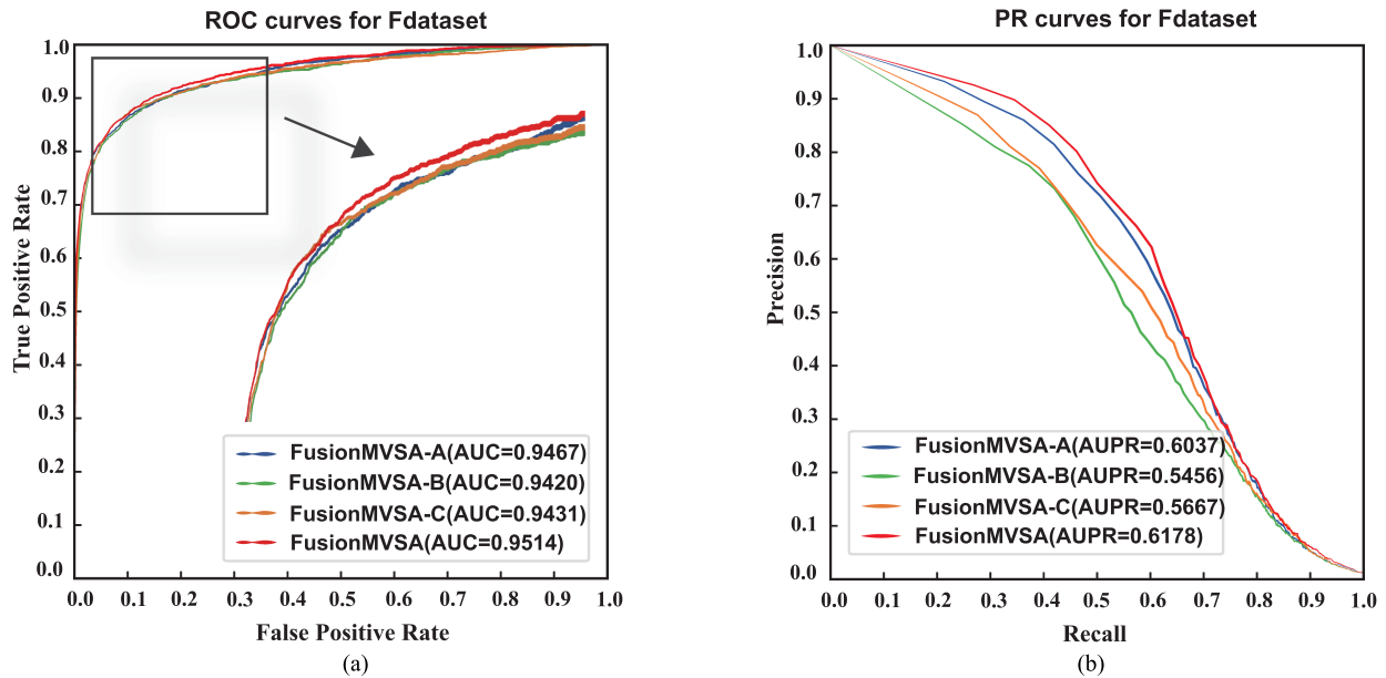
Fig. 3. Performance of FusionMVSA and other three variants in 10-fold cross-validation on Fdataset. (A) Receiver operating characteristic (ROC) curves of FusionMVSA and its variants. (B) Precision-recall (PR) curves of FusionMVSA and its variant.
