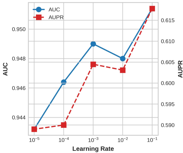
Fig. 2. Impact of different learning rates on model performance.
