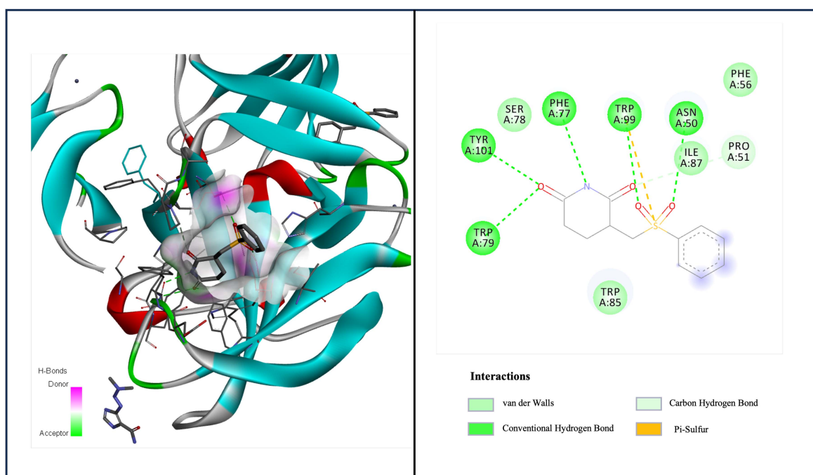
Fig. 4. Docked Dacarbazine (DrugBank ID: DB00851) with (PDB code:8AQO) as well as their interactions.
